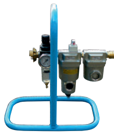
Combined filter on support frame F 056
